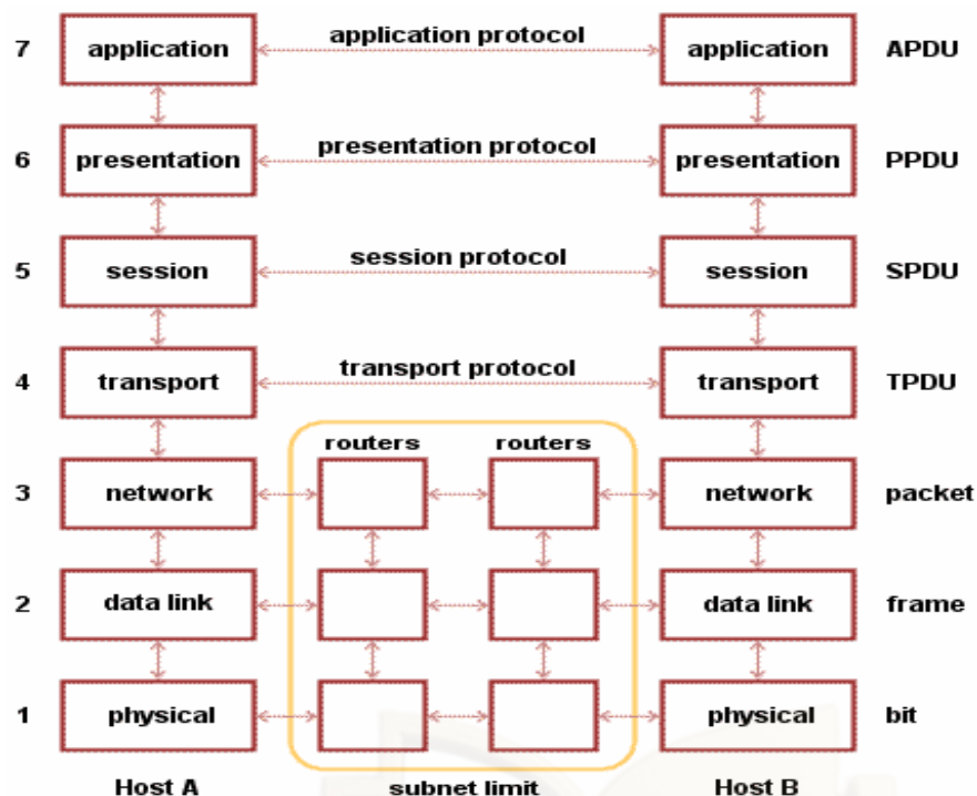
Figure 5.7: OSI Layer
