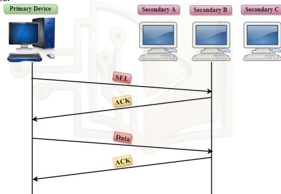
Figure 8.28: Select
