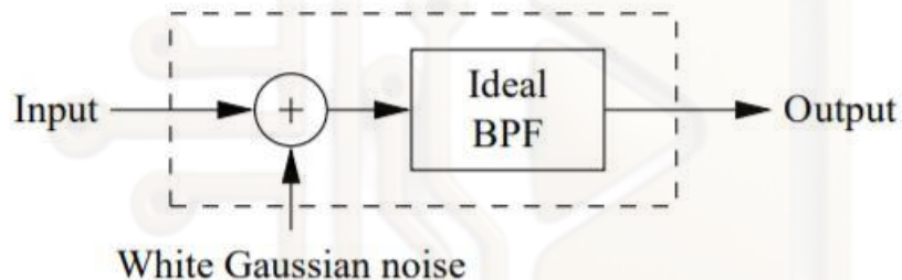
Figure 3.13: Shannon-Hartley Theorem
