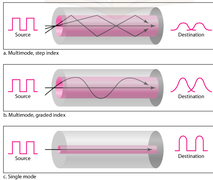
Figure 9: Modes of propagation
