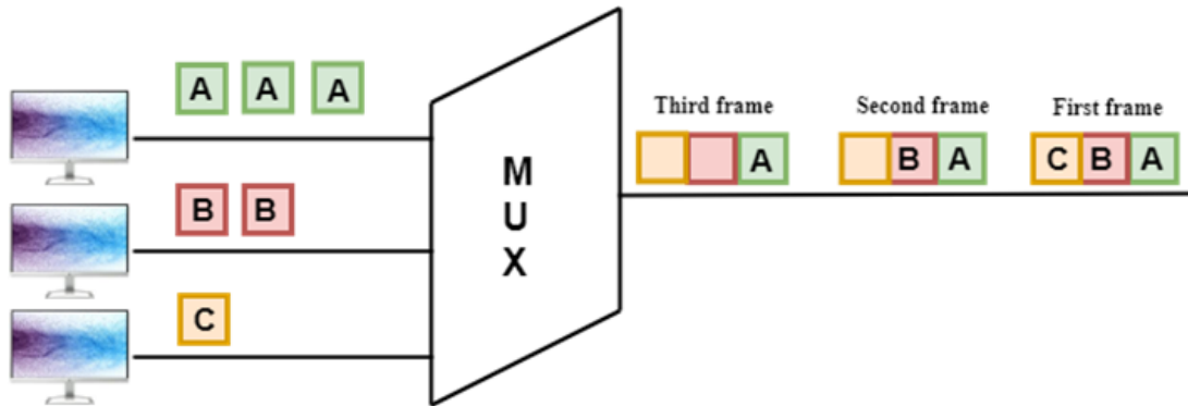
Figure 9.38: Synchronous TDM
