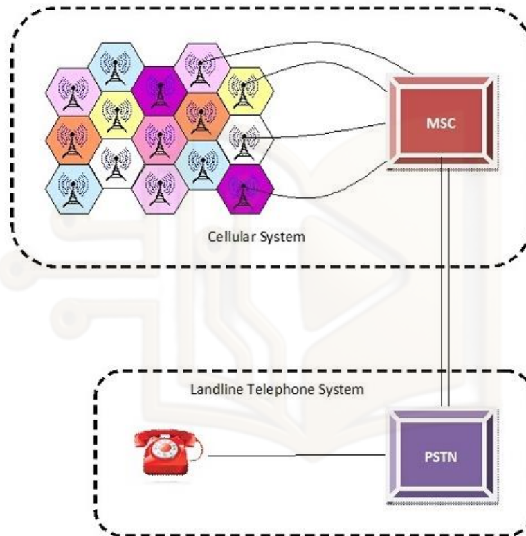
Figure 9.12: Switching Center
