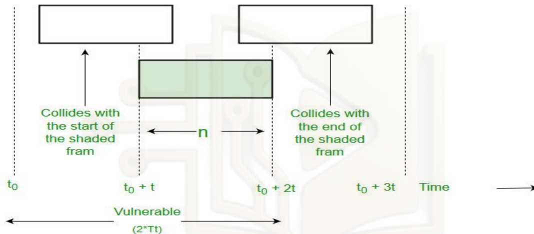
Figure 5.10: Pure Aloha
