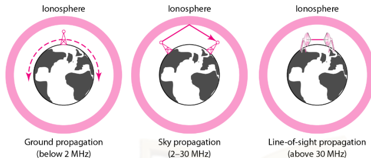
Figure 10: Propagation Method
