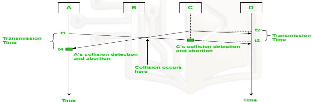
Figure 5.13: CSMA/ CD
